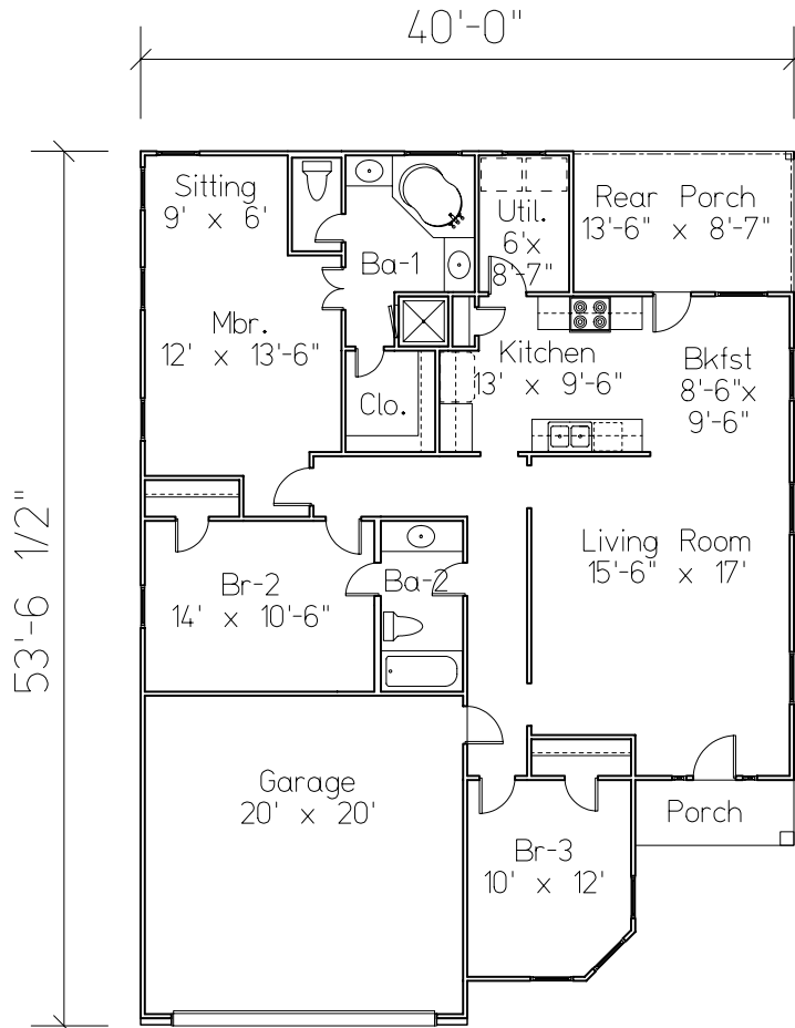
Floor Plan
