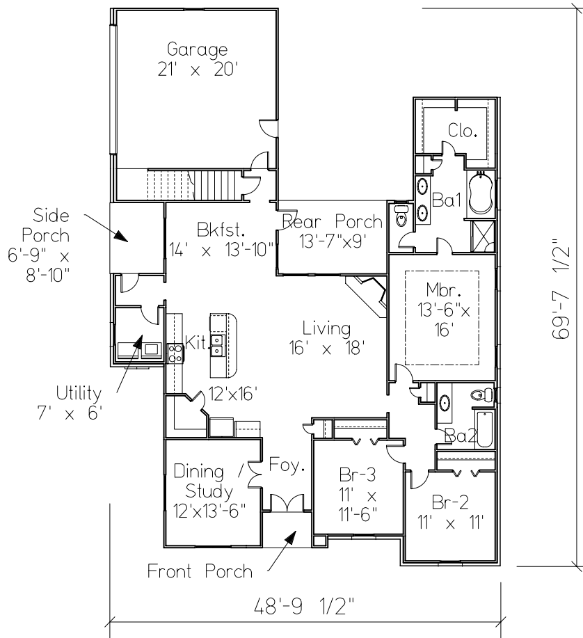
Lower Level Floor Plan
