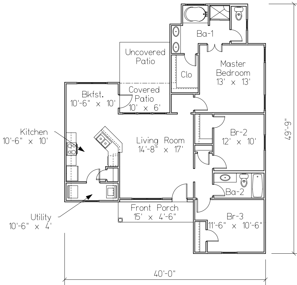
Floor Plan
